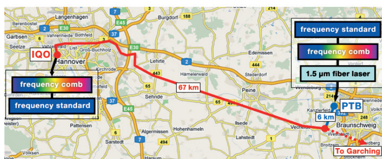
Figure 8: Schematic of a comparison of remote frequency standards by means of a link based on dark telecommunication fibers (blue and red lines). The dashed line indicates a planned extension (see text). At PTB a 1.5\text{ }\mu\text{m} fiber laser is locked to an optical frequency standard. Its output is transmitted to Leibniz Universität Hannover where its frequency is compared with that of an optical frequency standard based on Magnesium atoms. (Map source: Google Maps)
