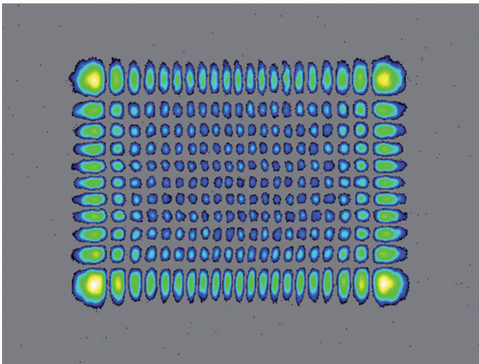
Figure 13: Image of a \text{TEM}_{20,10} light beam generated by a spatial optical phase modulator. The excitation of such high-order modes in a reference cavity reduces the effect of thermal noise in comparison with \text{TEM}_{00} excitation because thermal fluctuations are averaged over a larger area.
