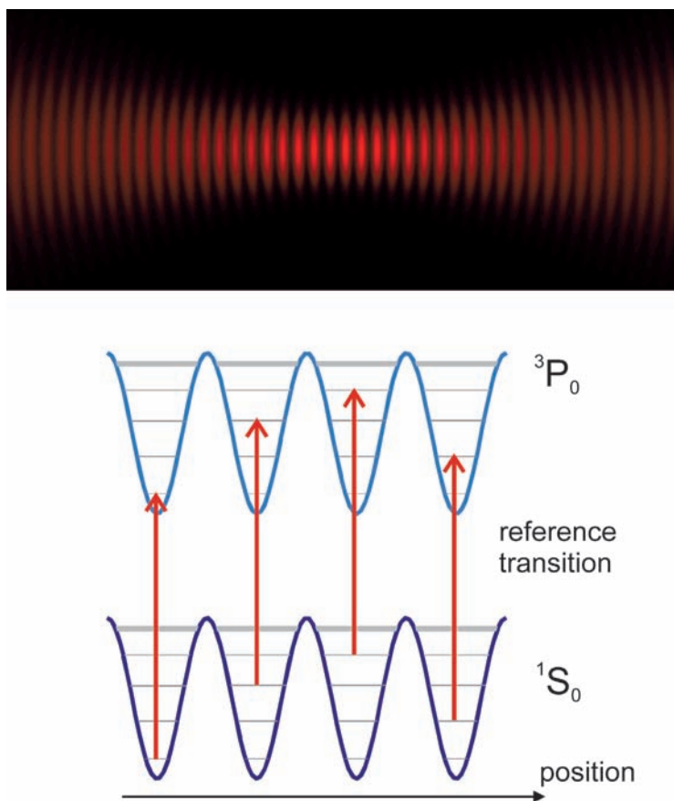
Figure 8: The most simple optical lattice is made from the standing wave of a retroreflected laser beam. Intensity distribution (top) and potential for both levels of the atomic reference transition (bottom).
